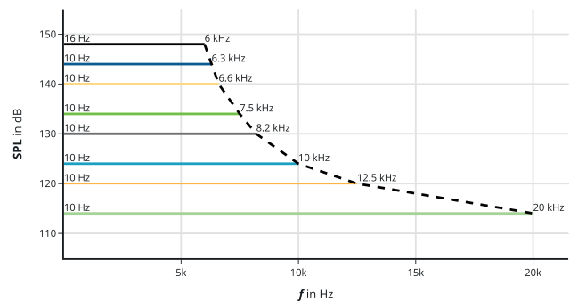
▲ Maximum performance with optional amplifier and both capsules LS-adapted
