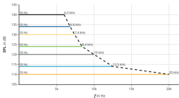
▲ Standard amplifier and both capsules LS-adapted
