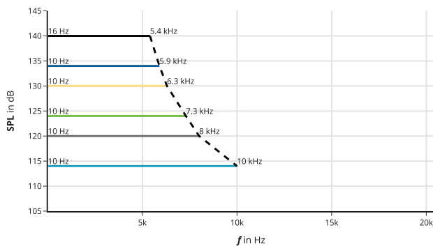
▲ Standard amplifier and both capsules with protection grid
