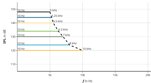
▲ Maximum performance with optional amplifier and both capsules with protection grid
